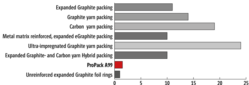
Weight loss in % after the exposure to temperature of 600 °C in stuffingbox
